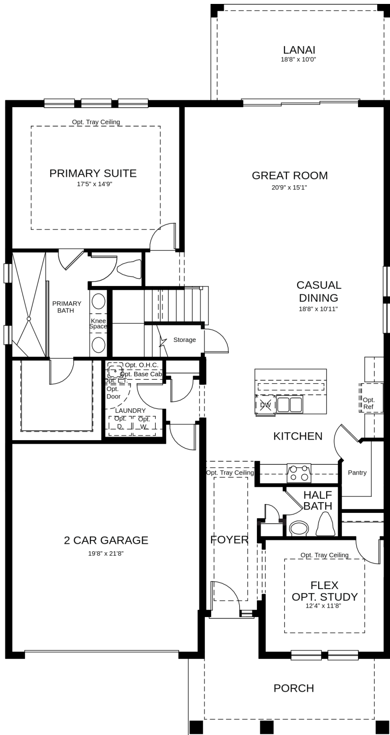
First Floor
